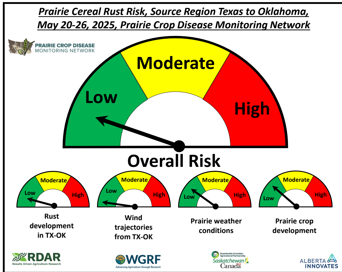
Figure. 19. Prairie cereal risk speedometers for stripe/leaf rust from the Texas to Oklahoma region, May 20-26, 2025.
