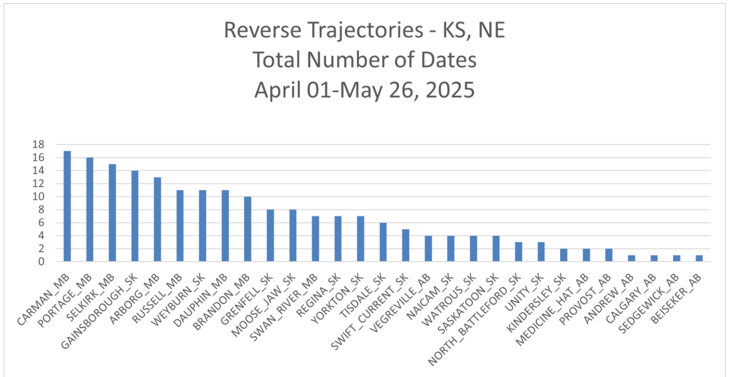
Figure 12. Reverse trajectory locations and number of events, for reverse trajectory events originating from Kansas and Nebraska, USA, April 1 – May 26, 2025.
