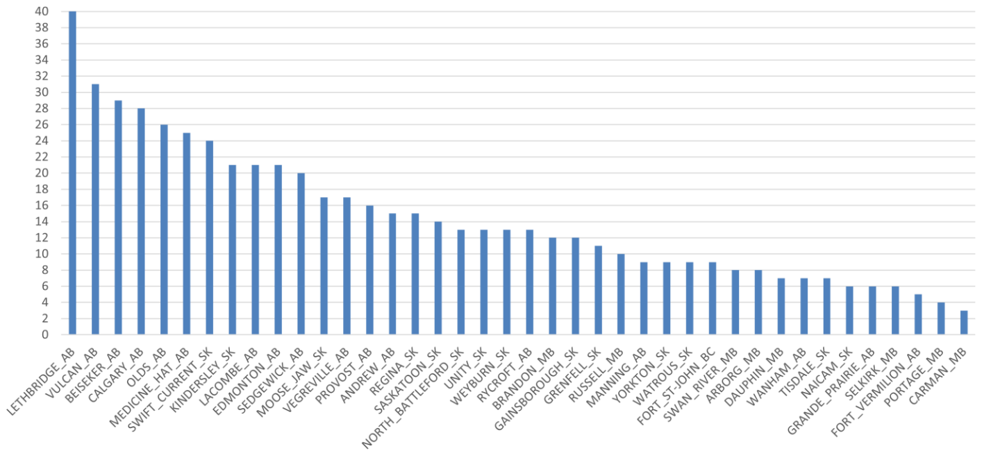
Figure 7. Reverse trajectory locations and number of events, for reverse trajectory events originating from the Pacific Northwest region of the USA, April 1 – May 26, 2025.
