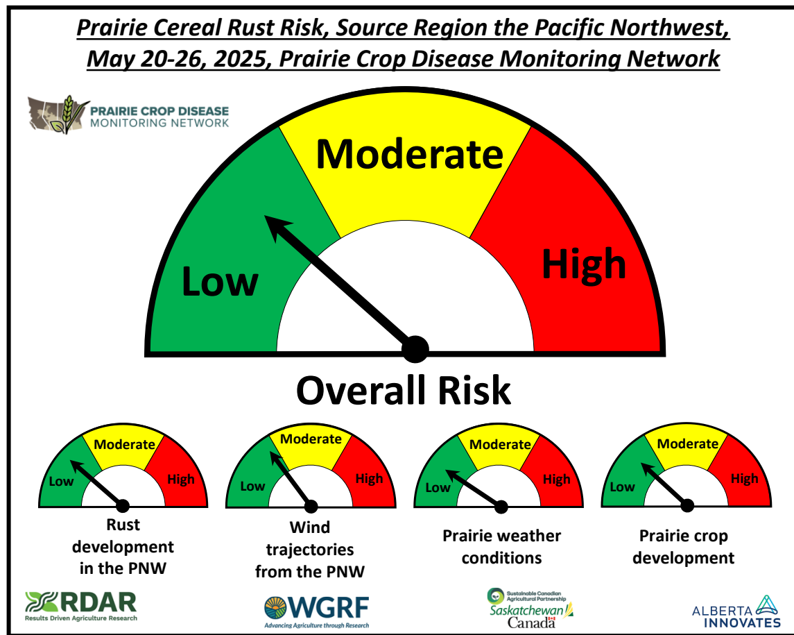
Figure 18. Prairie cereal risk speedometers for stripe rust from the Pacific Northwest, May 20-26, 2025.
