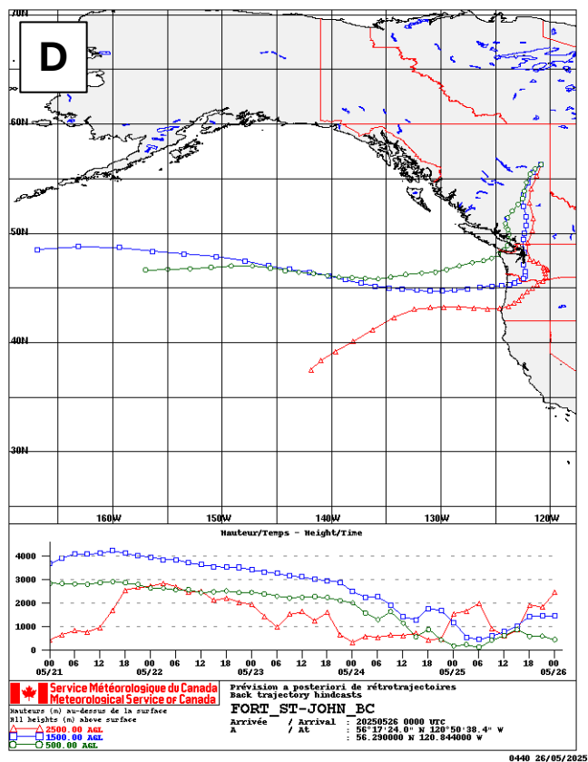
Figure 9a-d. Wind trajectory maps from Environment Canada for Manning, AB (A), Grande Prairie, AB (B), Fort Vermilion, AB (C), and Fort St. John, BC (D) for May 26, 2025.
