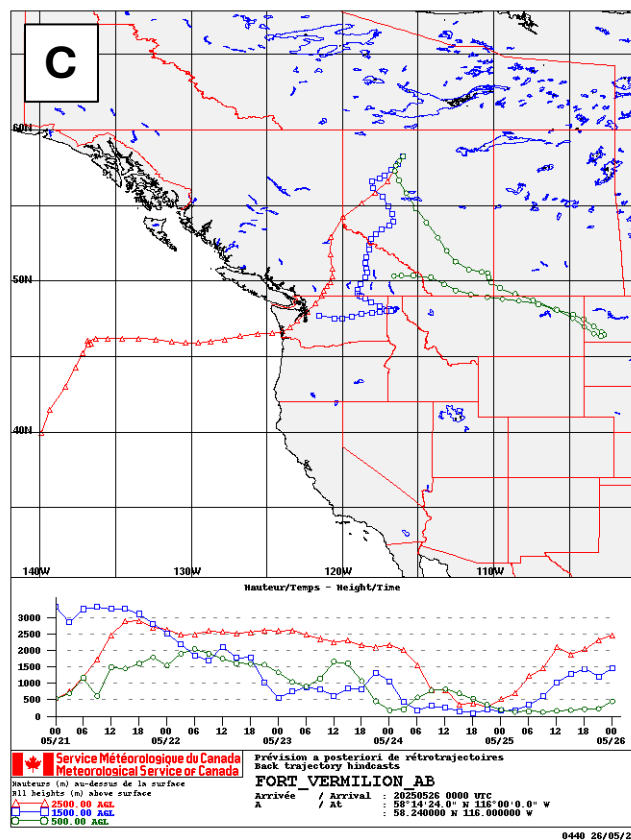
Figure 9a-d. Wind trajectory maps from Environment Canada for Manning, AB (A), Grande Prairie, AB (B), Fort Vermilion, AB (C), and Fort St. John, BC (D) for May 26, 2025.
